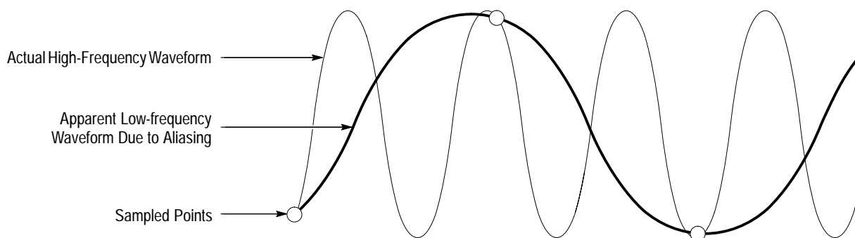
Figure 3–18: Aliasing
