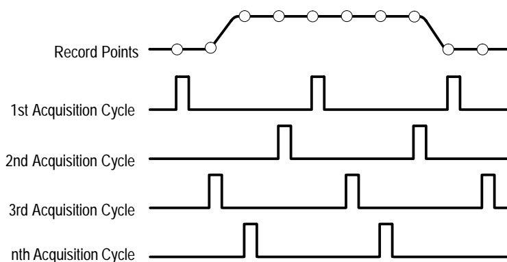
Figure 3–14: Equivalent-Time Sampling
