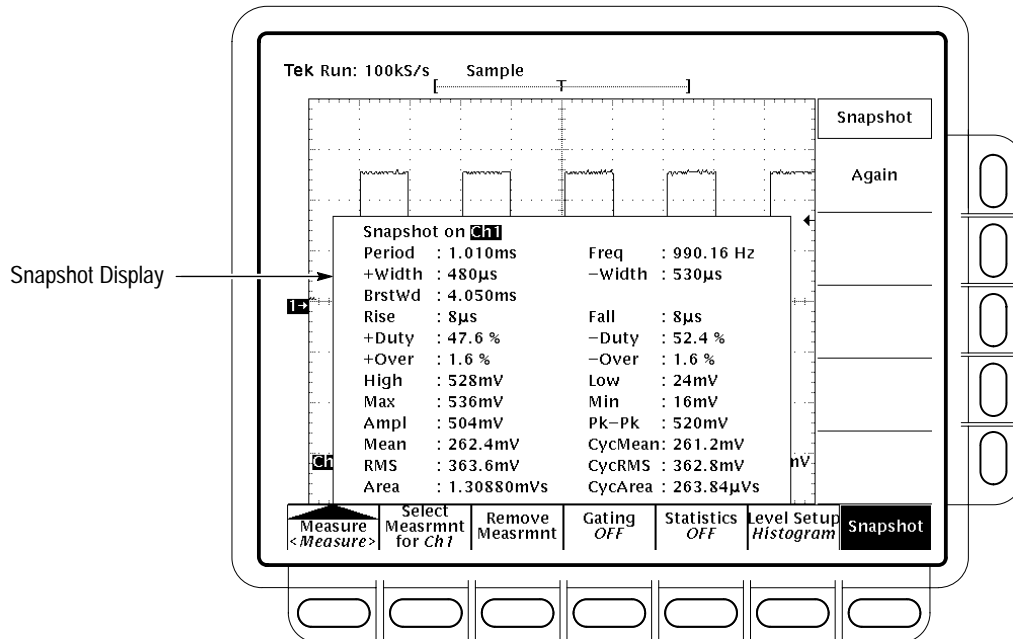
Figure 3-60: Snapshot Menu and Readout
